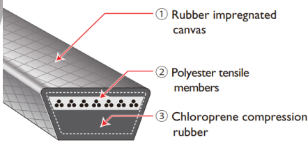
RED-S II V-belt
